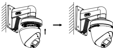
Figure 2-23 Finish Installation
