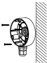
Figure 2-4 Secure Junction Box on Wall
