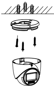
Figure 2-7 Secure Base to Ceiling
