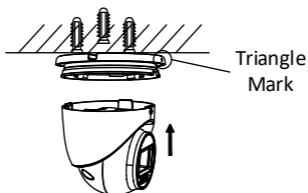
Figure 2-8 Install Camera Back
