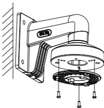
Figure 2-22 Fix Installation Plate
