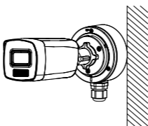
Figure 2-5 Fix Cover to Its Body
