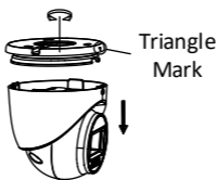
Figure 2-6 Disassemble Camera
