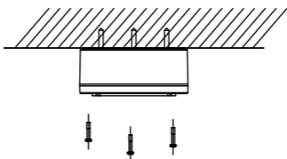
Figure 2-11 Combine Junction Box Cover and Body
