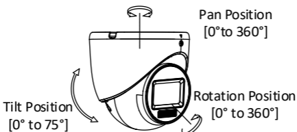
Figure 2-9 3-Axis Adjustment
