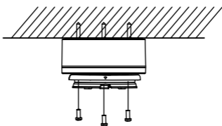
Figure 2-12 Fix Base
