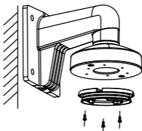
Figure 2-16 Fix Base onto Wall Mount
