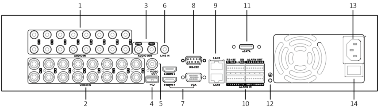
Figure 1-31 Rear Panel of DS-8100HTHI-K8
